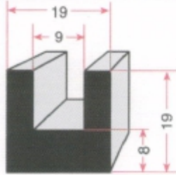
U LASTİĞİ GRP 0937
